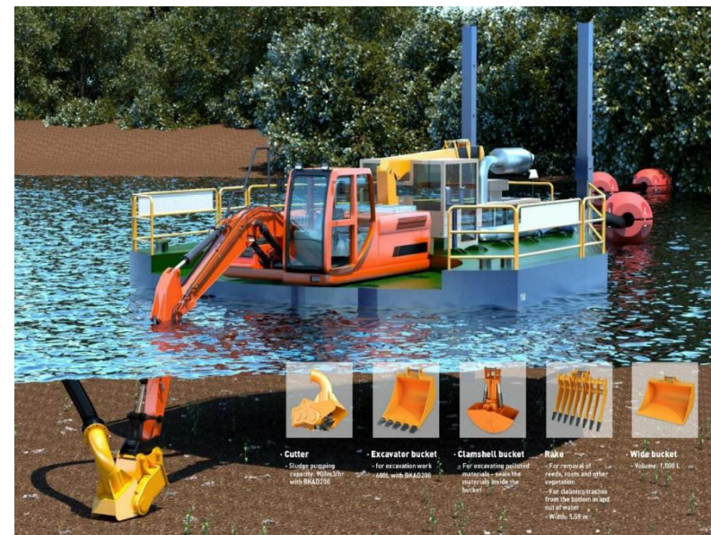
AMPHIBIOUS DREDGER SERIES BKAD 150/200/250/250/300
