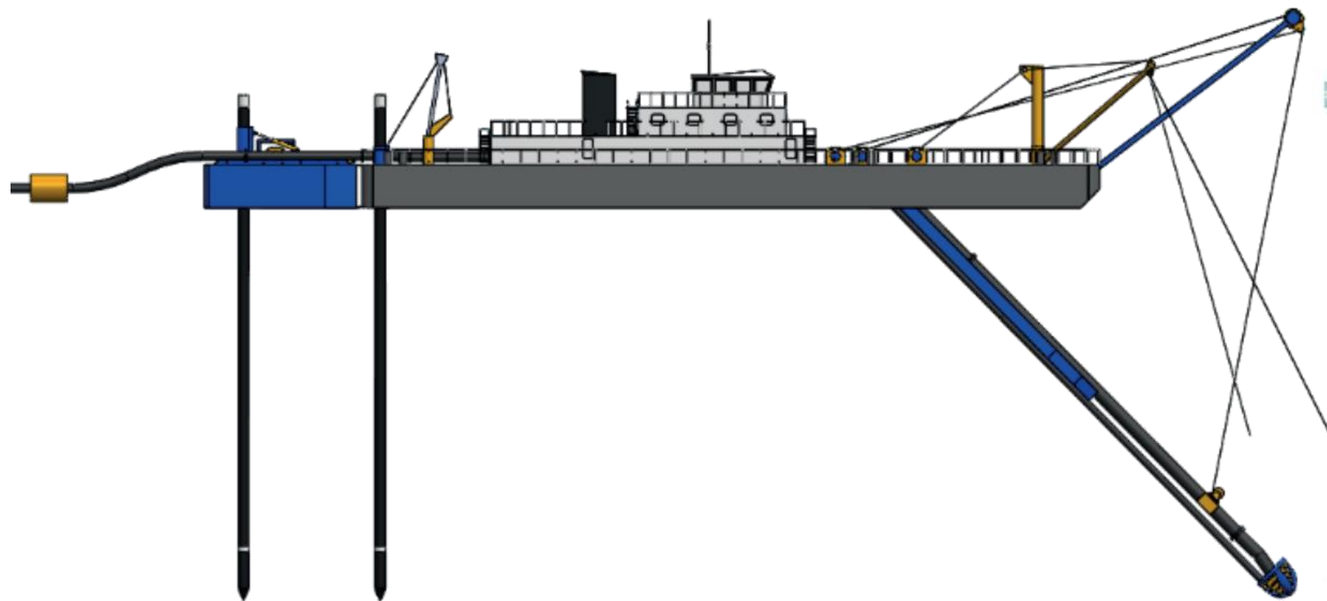
CSD(Cutter Suction Dredger)
